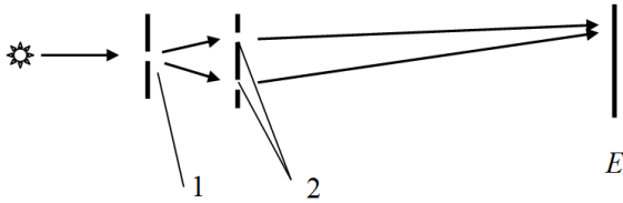
Figure 1.1 – Light from a source is incident on the screen through two slits
